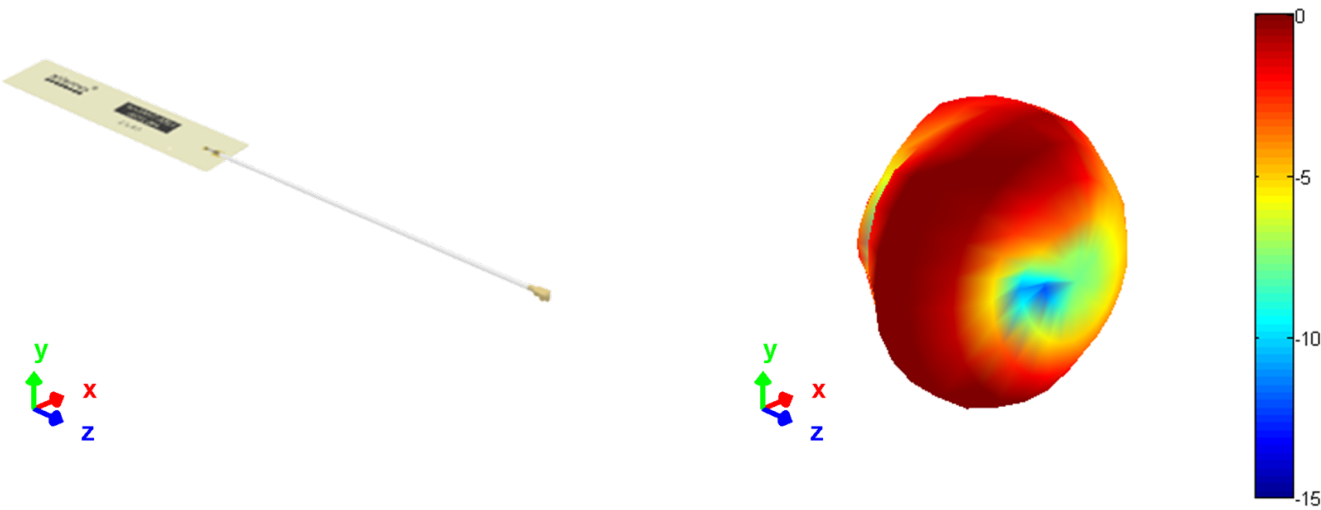
3D pattern at 900MHz
