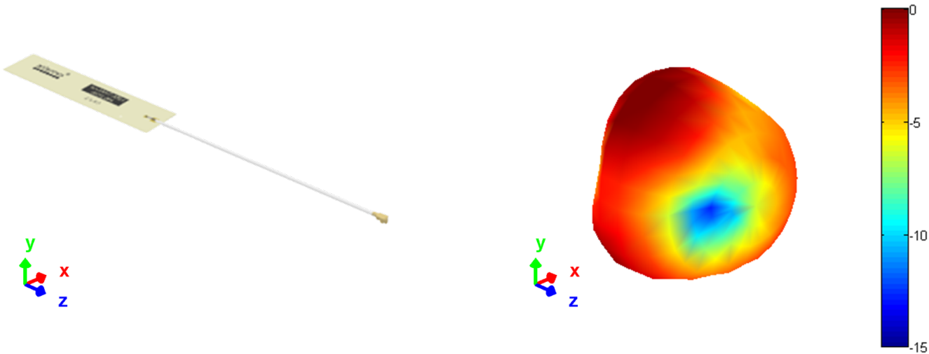
3D pattern at 657MHz
