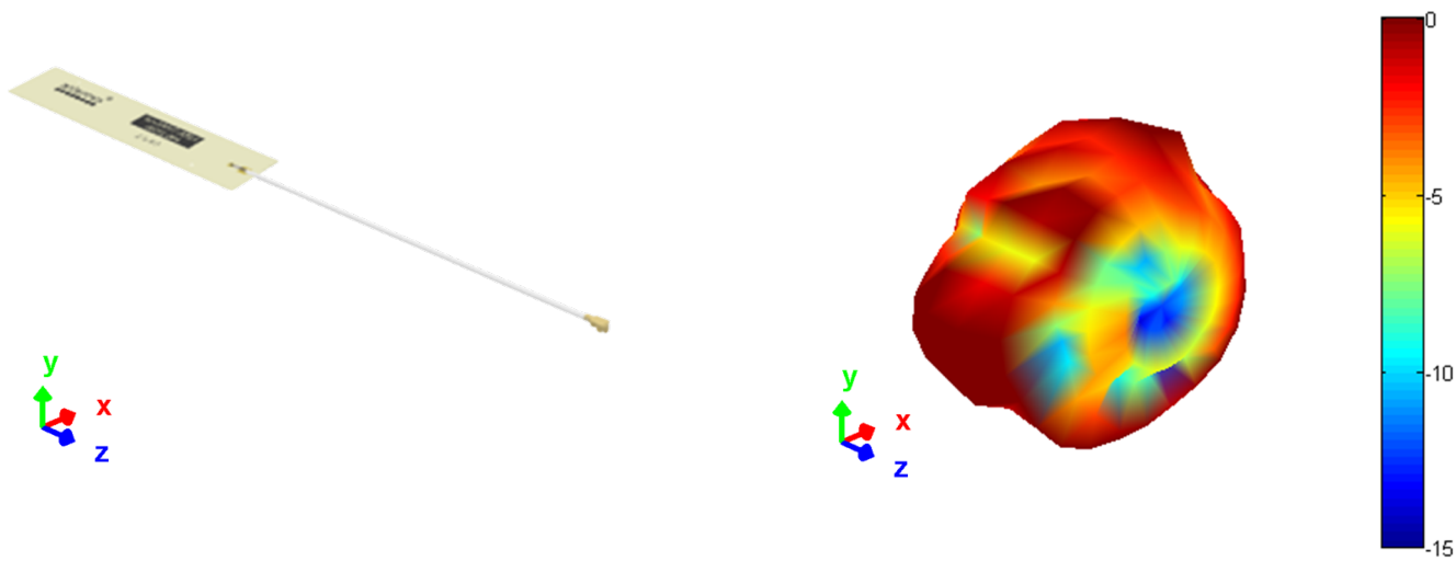
3D pattern at 2600MHz
