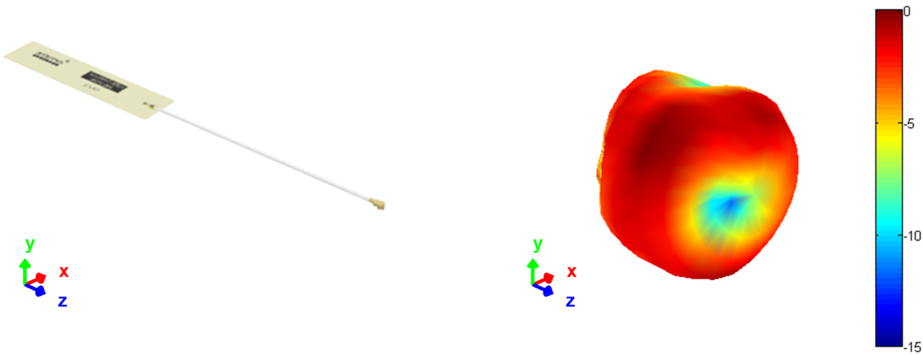
3D pattern at 764MHz
