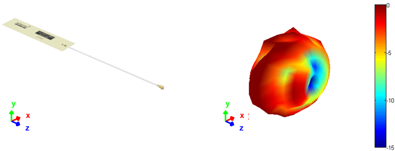
3D pattern at 1930MHz
