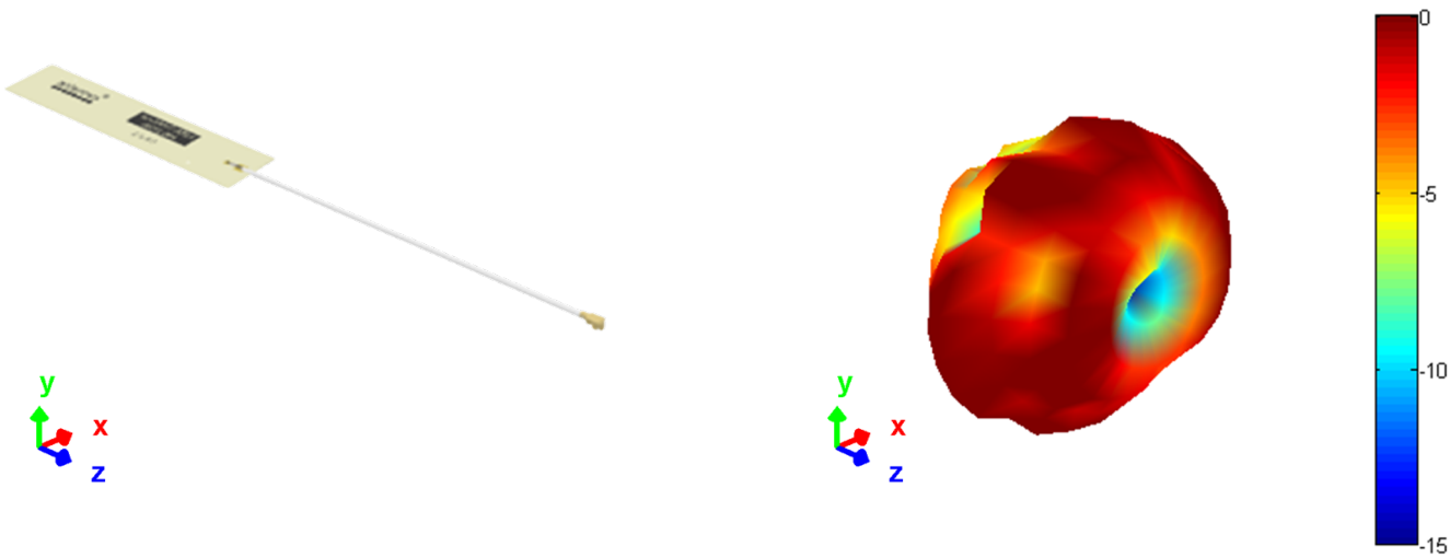
3D pattern at 2340MHz
